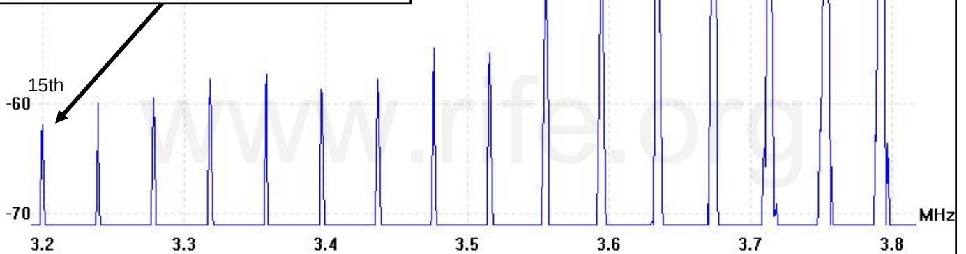
Philip Hoyland's Beam Ray Clinical instrument 3.80 Megahertz spectrum analysis of sideband harmonic frequencies.
