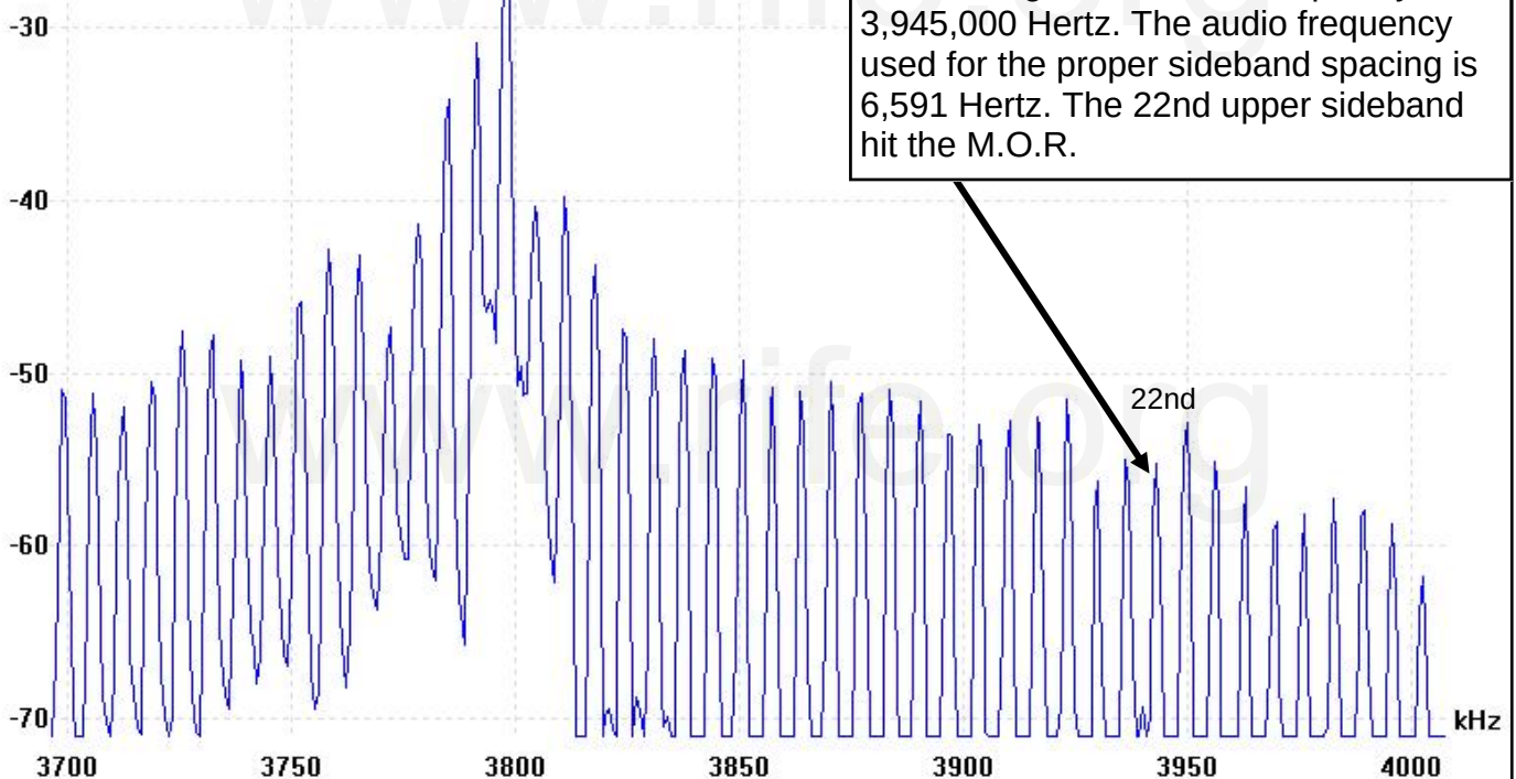
Philip Hoyland's Beam Ray Clinical instrument 3.80 Megahertz spectrum analysis of sideband harmonic frequencies.
